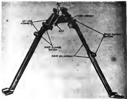
Figure 50 M2 bipod
